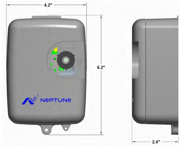
Figure 5 – Wall Cellular Endpoint with External Antenna – Dimensions Front and Side
